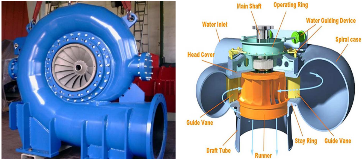
Figure 4.7: Turbines FRANCIS
