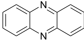
phenazine
