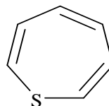
thiepine
